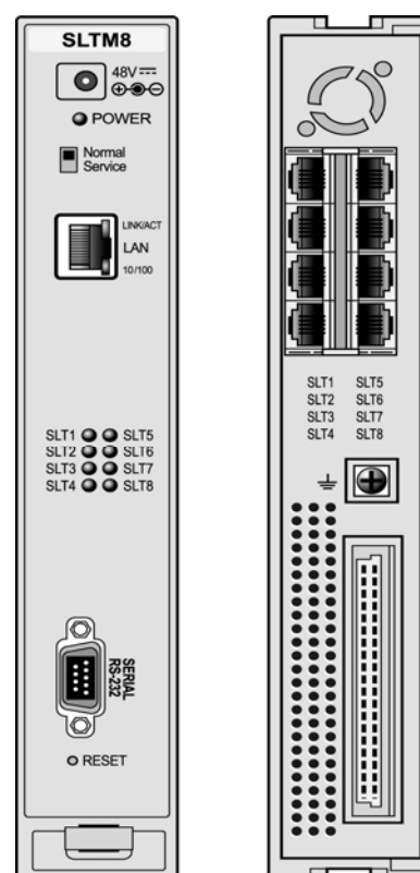
Figure 2.1.6.2-1 SLTM8 Front & Rear Panels
