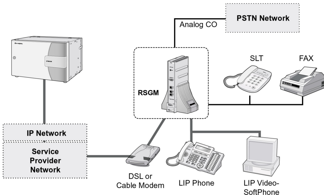
Figure 2.1.11-1 RSGM Connection
