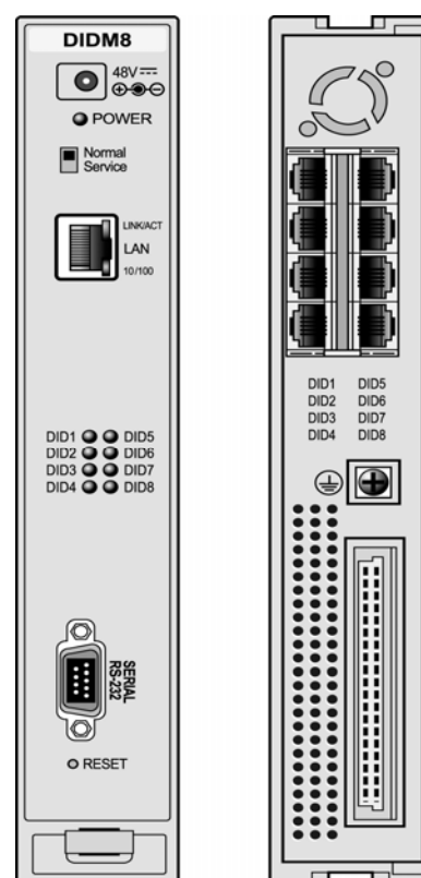
Figure 2.1.4-1 DIDM8 Front & Rear Panels
