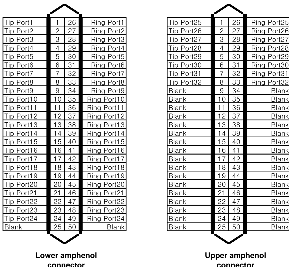
Figure 4.5.10-2 SLTM32 RJ-21X Connector Configuration
