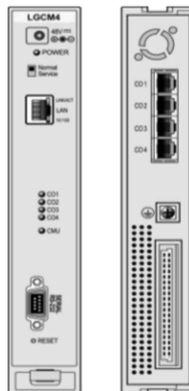
Figure 2.1.3.1-1 LGCM4 Front & Rear Panels
