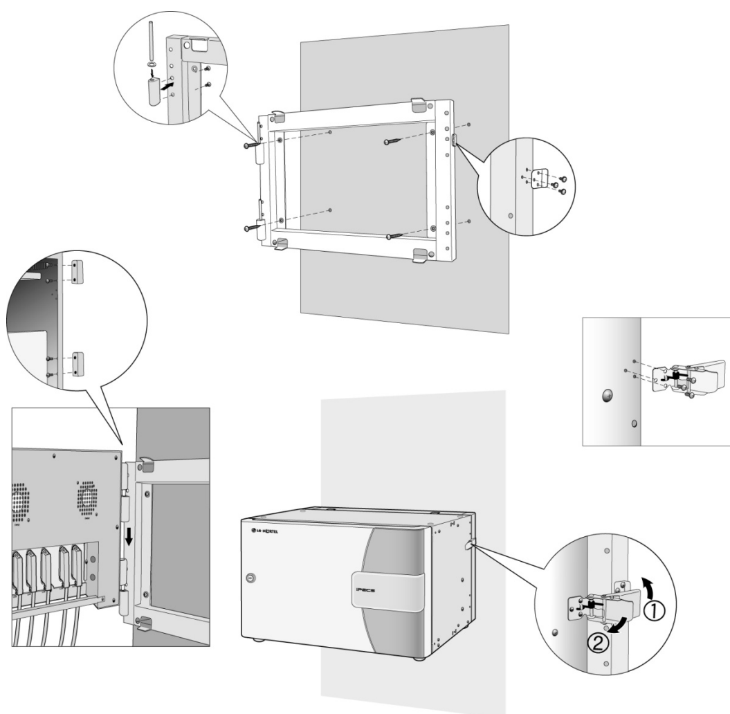
Figure 4.3.1.3-1 Cabinet Wall Mount Kit Installation
