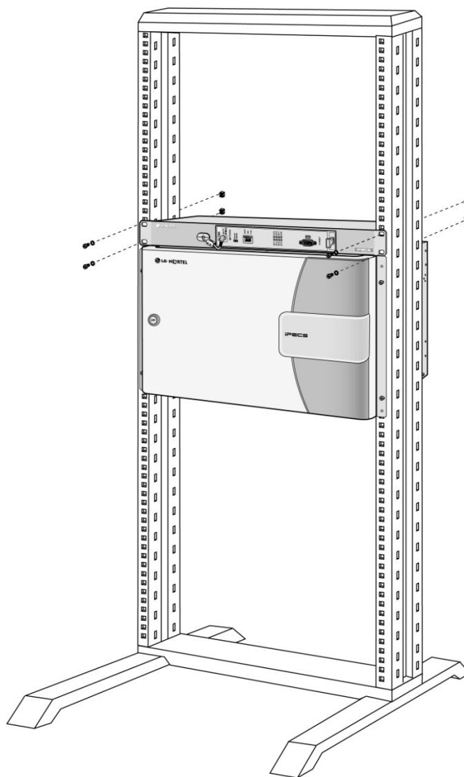
Figure 4.3.5-3 1U-RMB Rack-mount Installation
