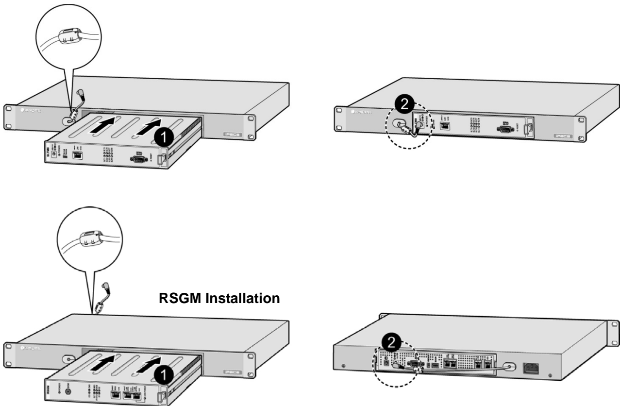
Figure 4.3.5-2 1U-RMB Gateway Installation
