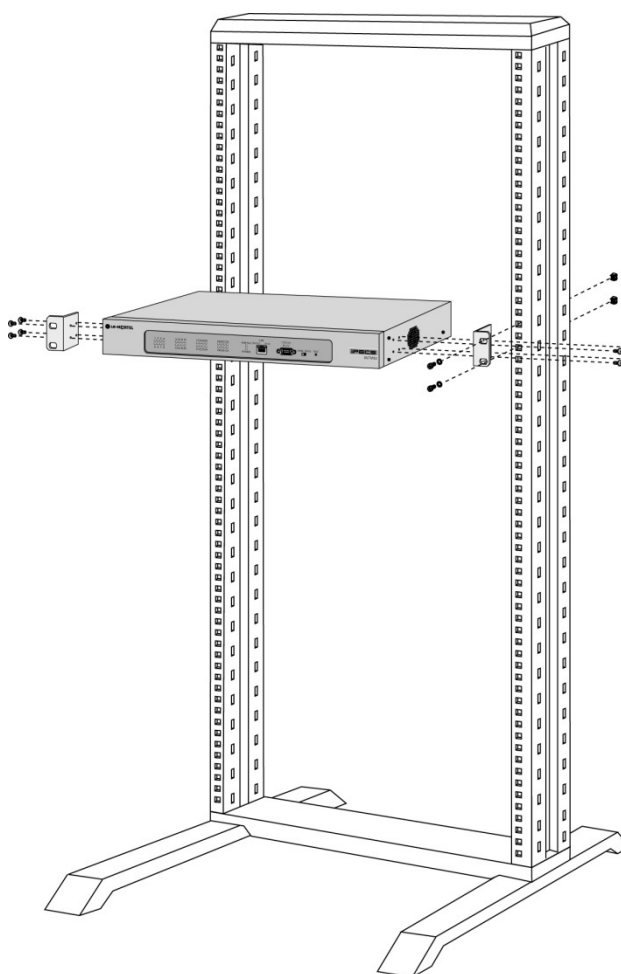
Figure 4.5.10-1 SLTM32 Rack Mounting Installation
