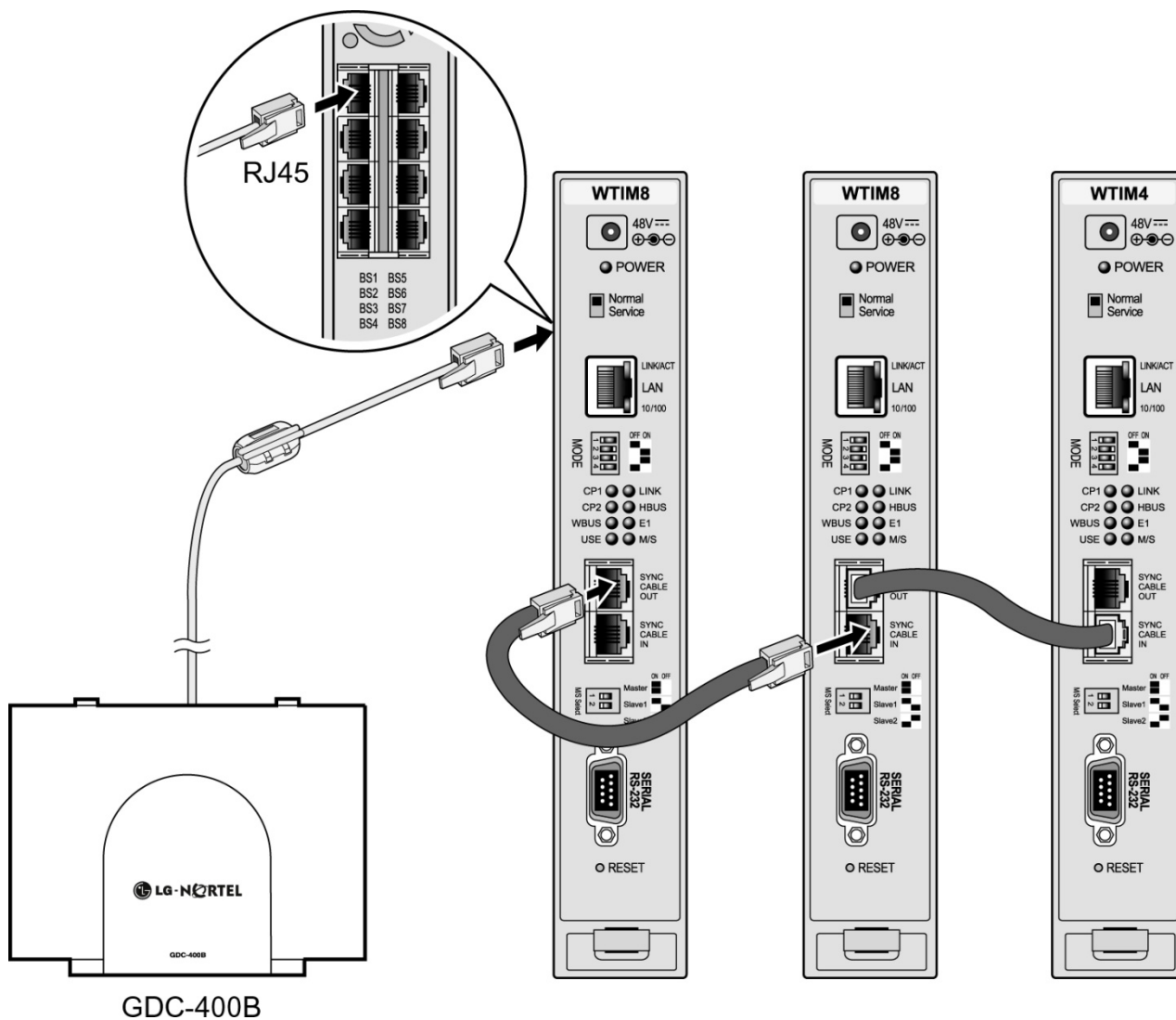
Figure 4.5.18-1 Cascading connections of WTIM4/8
