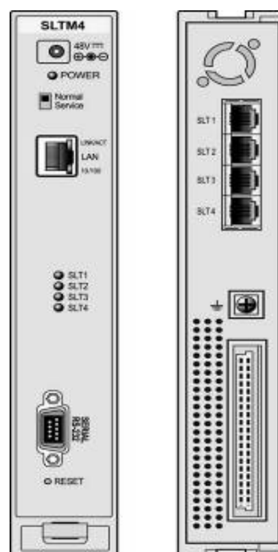
Figure 2.1.6.1-1 SLTM4 Front & Rear Panels
