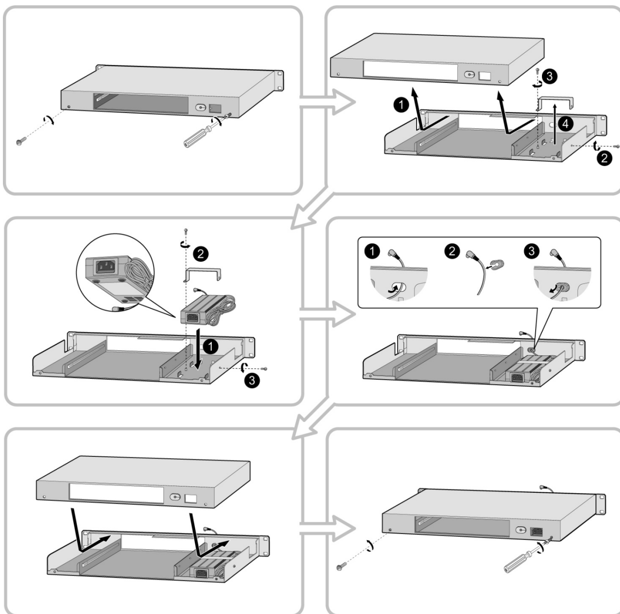
Figure 4.3.5-1 1U RMB Adapter Installation
