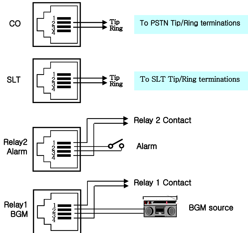
Figure 4.5.16-3 RSGM Connections
