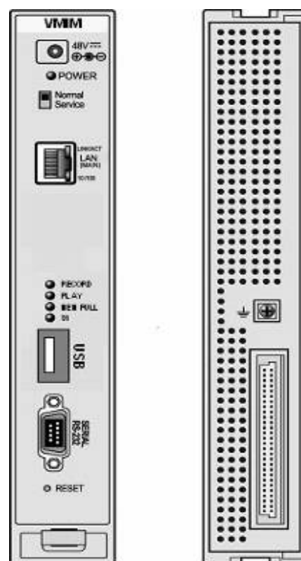
Figure 2.1.9-1 VMIM Front & Rear Panels
