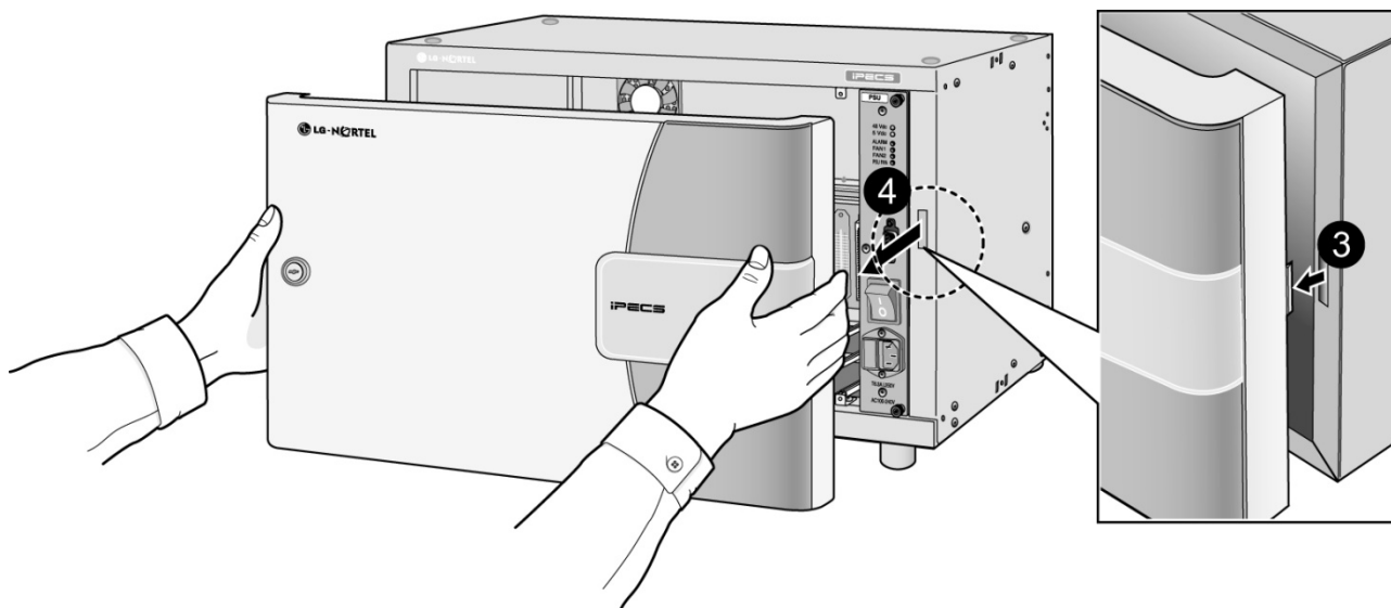
Figure 4.3.1.1-2 Cover removal
