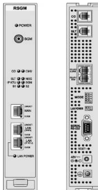
Figure 2.1.11-2 RSGM Front & Rear Panels
