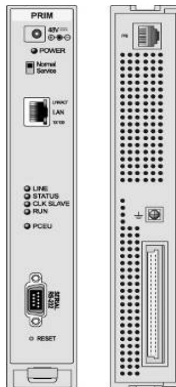
Figure 2.1.8-1 PRIM Front & Rear Panels
