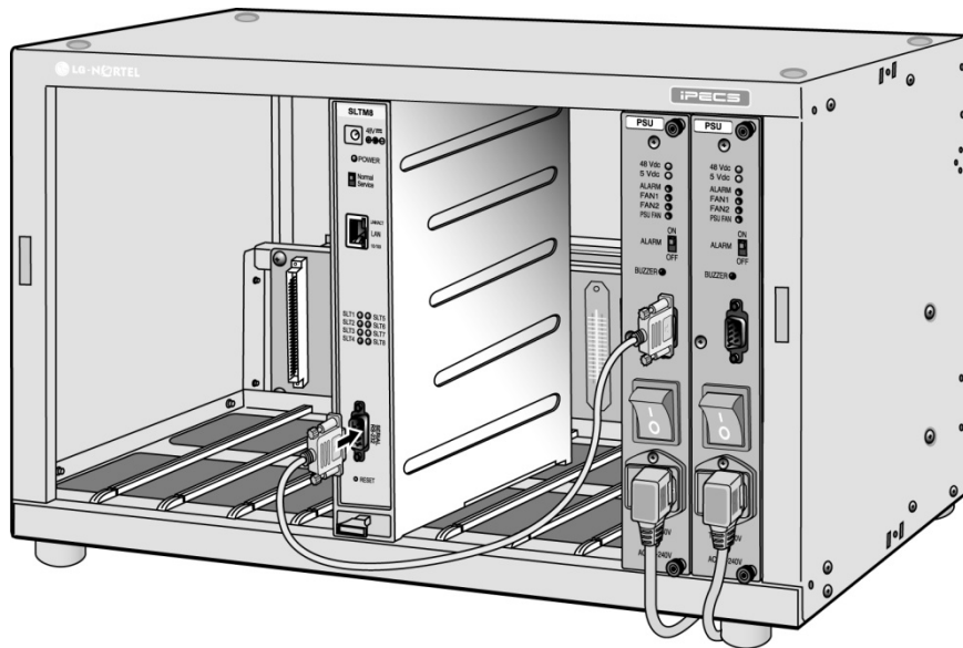
Figure 4.4-3 Monitoring cable Installation
