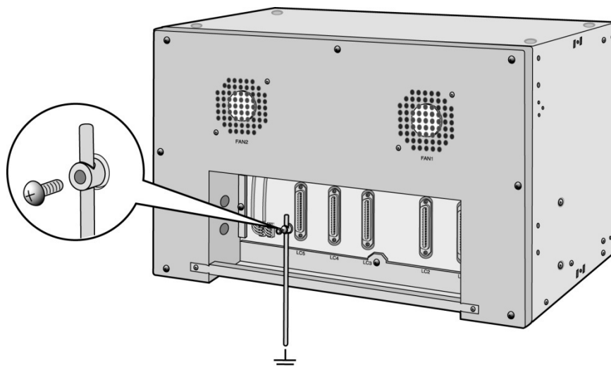
Figure 4.3.2-1 MCKTE Grounding
