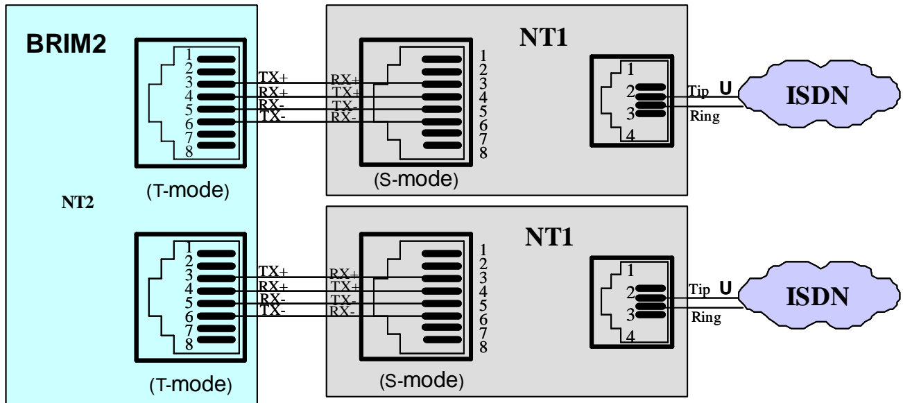
Figure 4.5.11-1 BRIM2 BRI Line Connector Configuration
