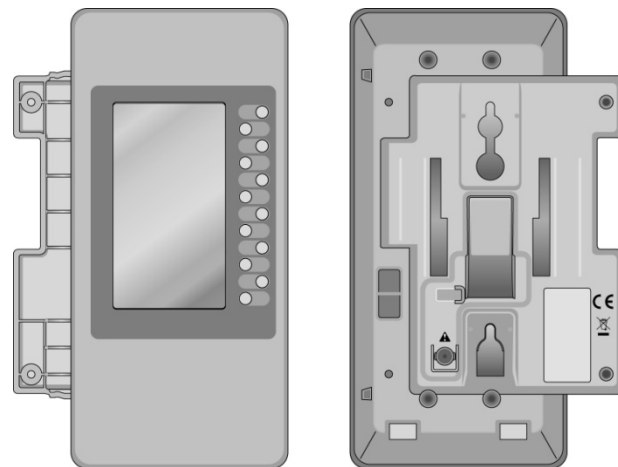
Figure 2.2.1-6 LIP-8012LSS
