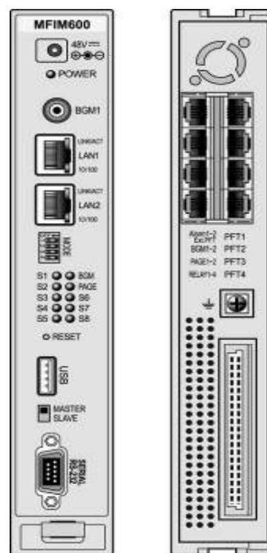
Figure 2.1.1-1 MFIM Front & Rear Panel Example
