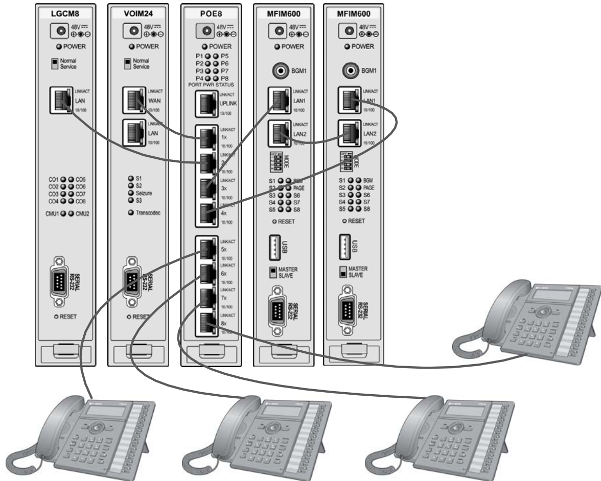
Figure 4.5.17-1 POE8 Installation
