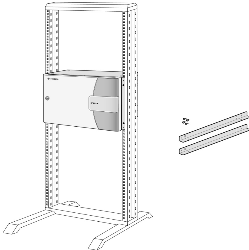
Figure 2.3.4-2 19" Rack Mount Installation
