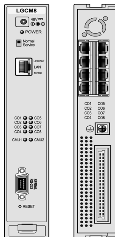
Figure 2.1.3.2-1 LGCM8 Front & Rear Panels
