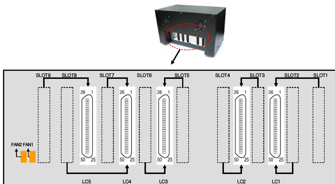
Figure 4.6-1 RJ-21x Connector Backplane Wiring Diagram
