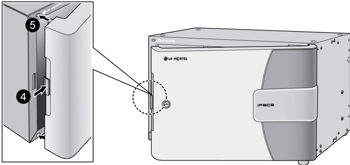
Figure 4.3.1.1-1 Cover installation
