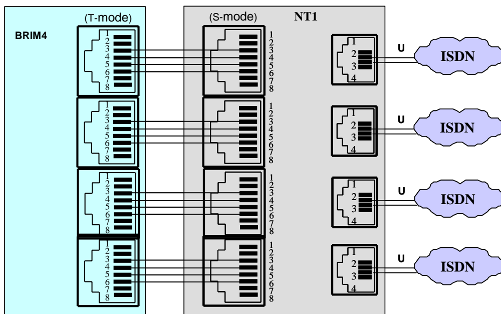
Figure 4.5.12-1 BRIM4 BRI Line Connector Configuration
