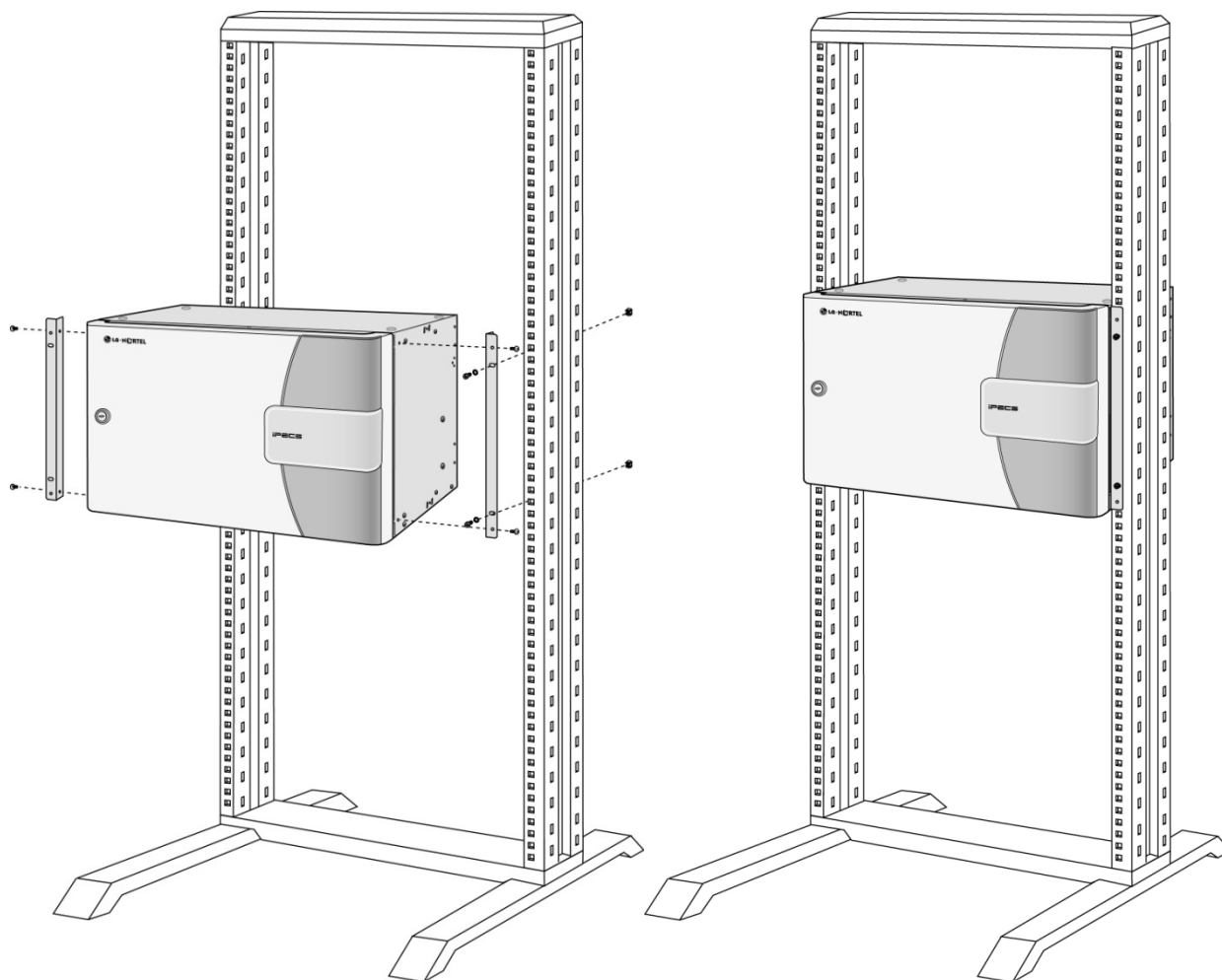
Figure 4.3.1.2-1 Rack (19") Installation
