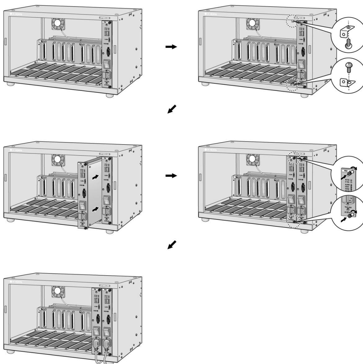
Figure 4.4-2 Back-up PSUs Installation
