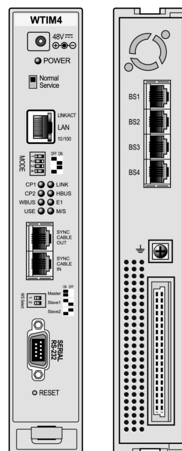
Figure 2.1.13.1-1 WTIM4 Front & Rear Panels
