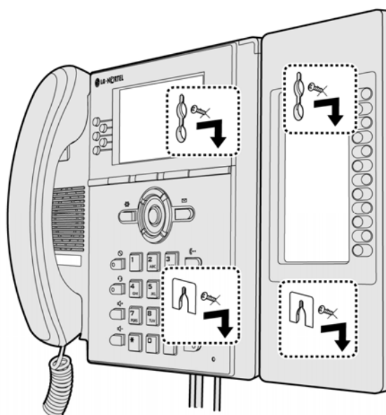
Figure 4.7-1 LIP-8000 Wall Mount Installation
