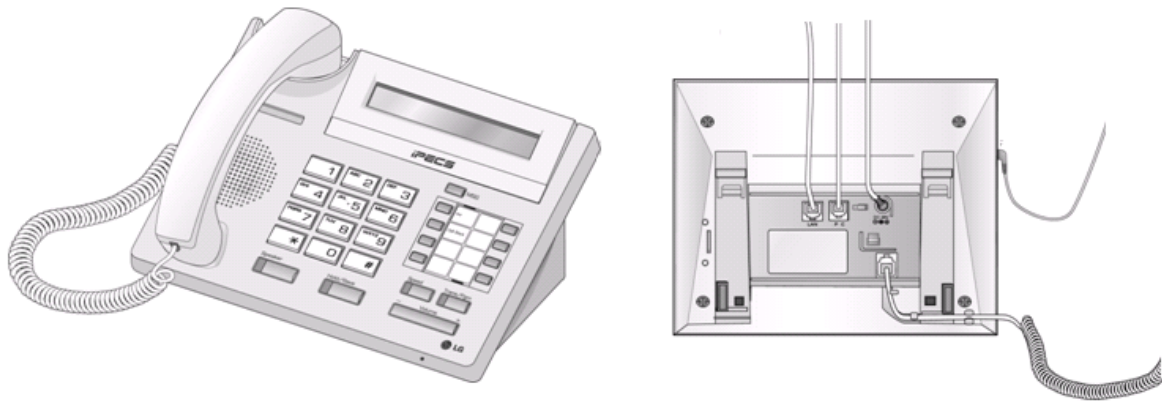
Figure 2.2.2-2 LIP-7008D
