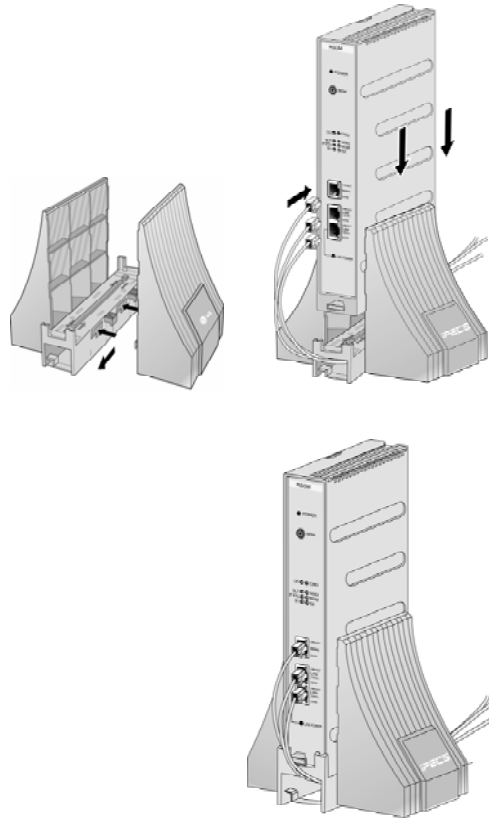
Figure 4.5.16-1 RSGM on Desk Mount Holder
