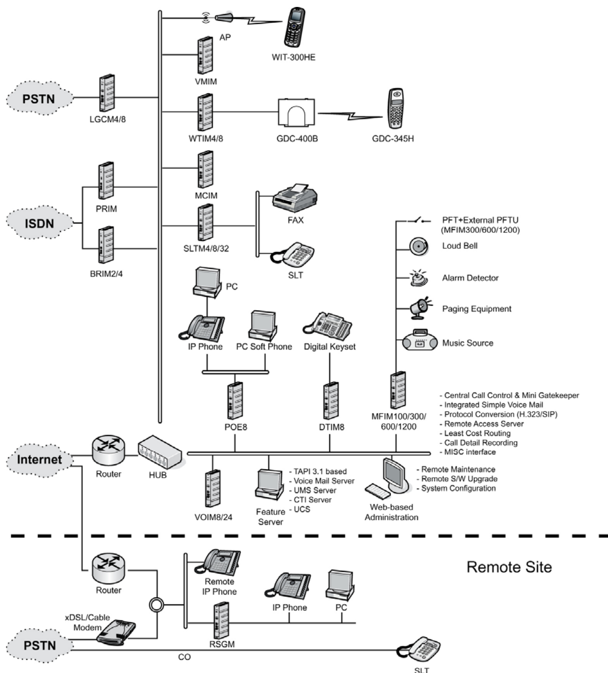
Figure 1.1-1 iPECS Structure
