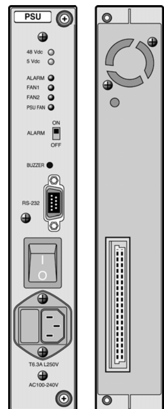
Figure 2.1.14-1 PSU Front & Rear Panels
