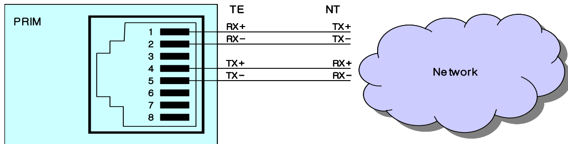
Figure 4.5.13-1 PRI Line Connector Configuration
