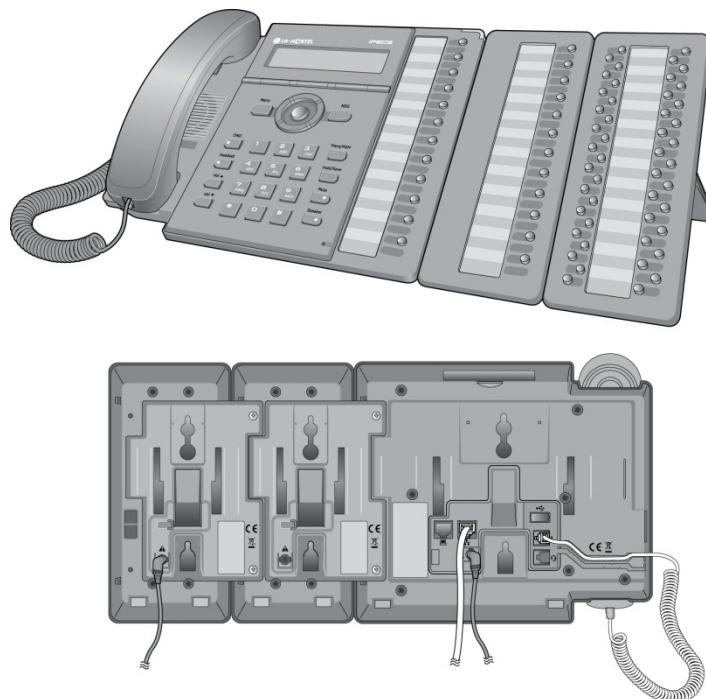
Figure 4.7-3 LIP-8000 DSS Installation (12DSS + 48DSS)
